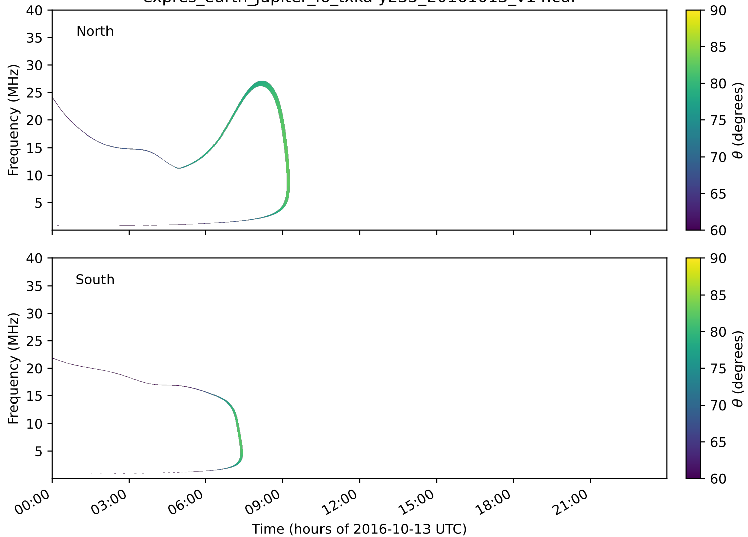
expres_earth_jupiter_io_txka-y235_20161013_v14.cdf
