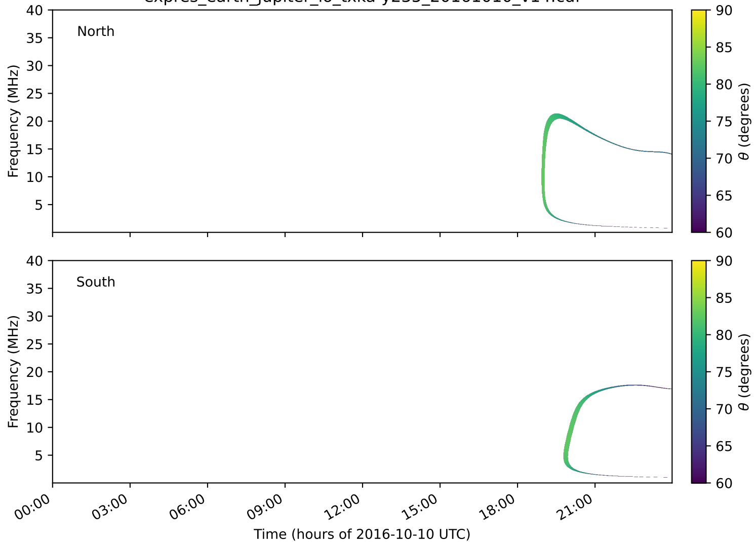
expres_earth_jupiter_io_txka-y235_20161010_v14.cdf
