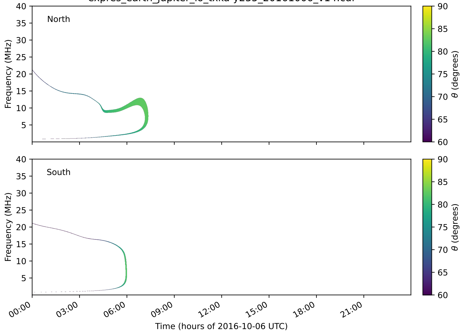
expres_earth_jupiter_io_txka-y235_20161006_v14.cdf
