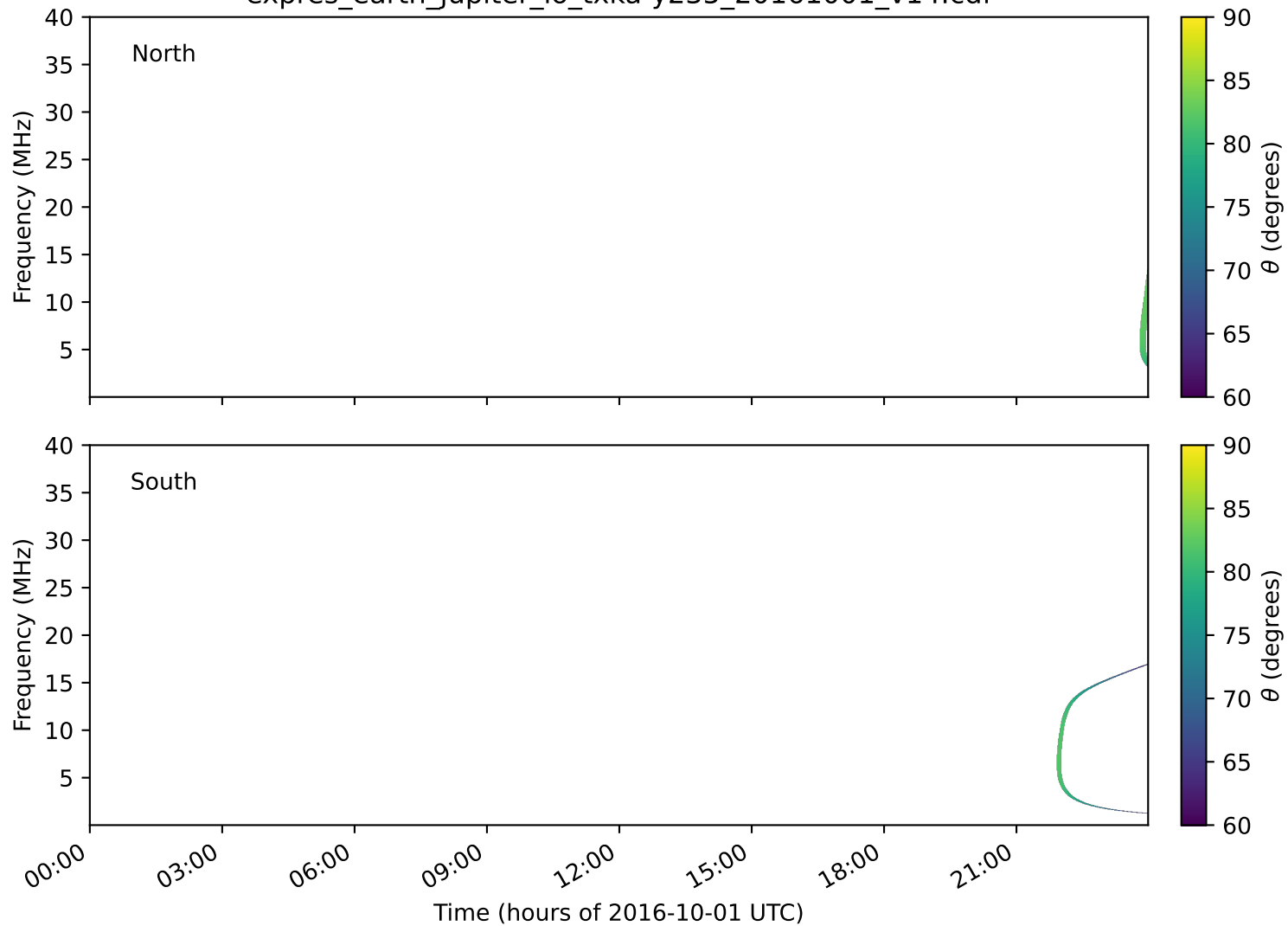
expres_earth_jupiter_io_txka-y235_20161001_v14.cdf
