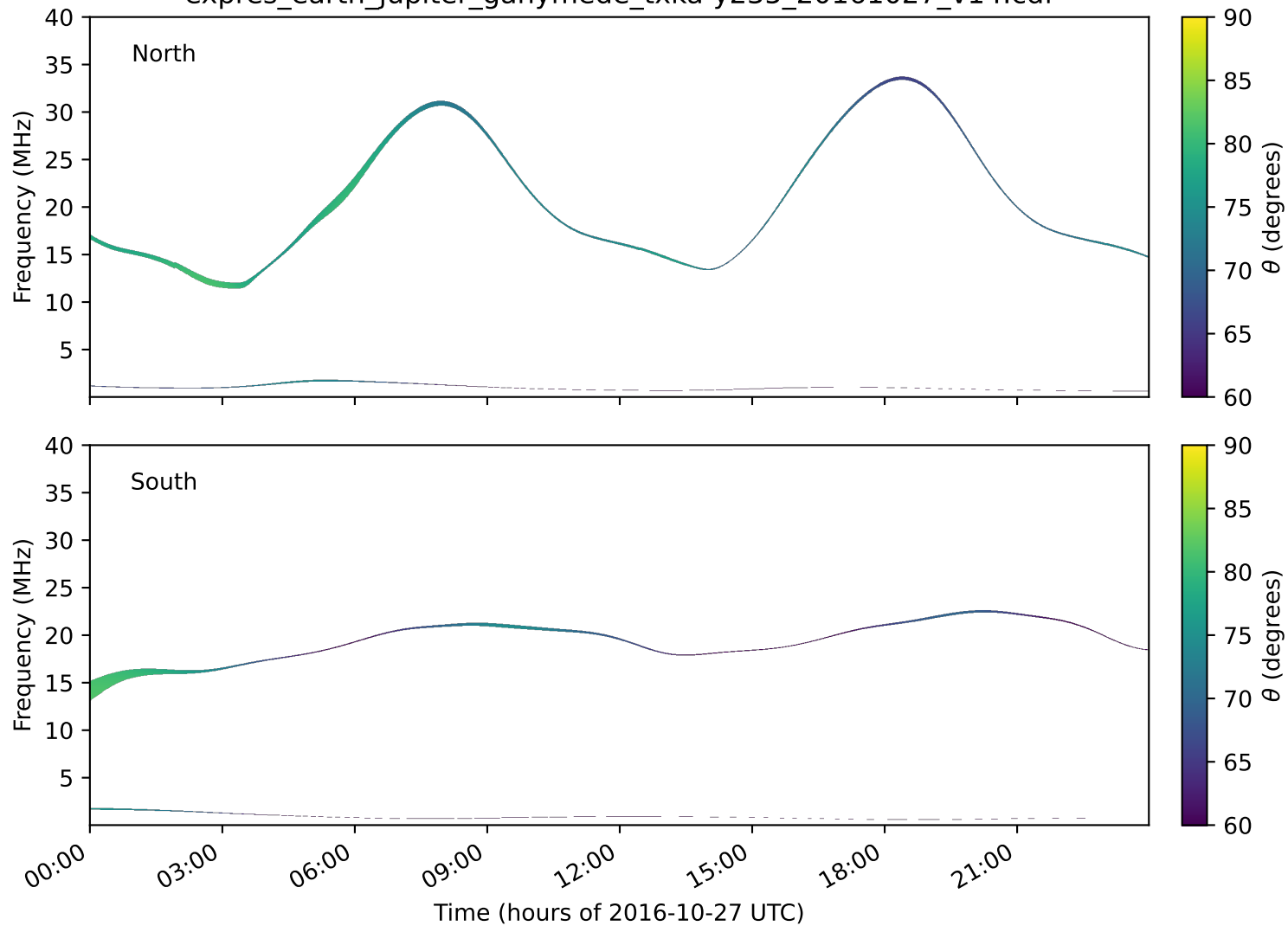
expres_earth_jupiter_ganymede_txka-y235_20161027_v14.cdf
