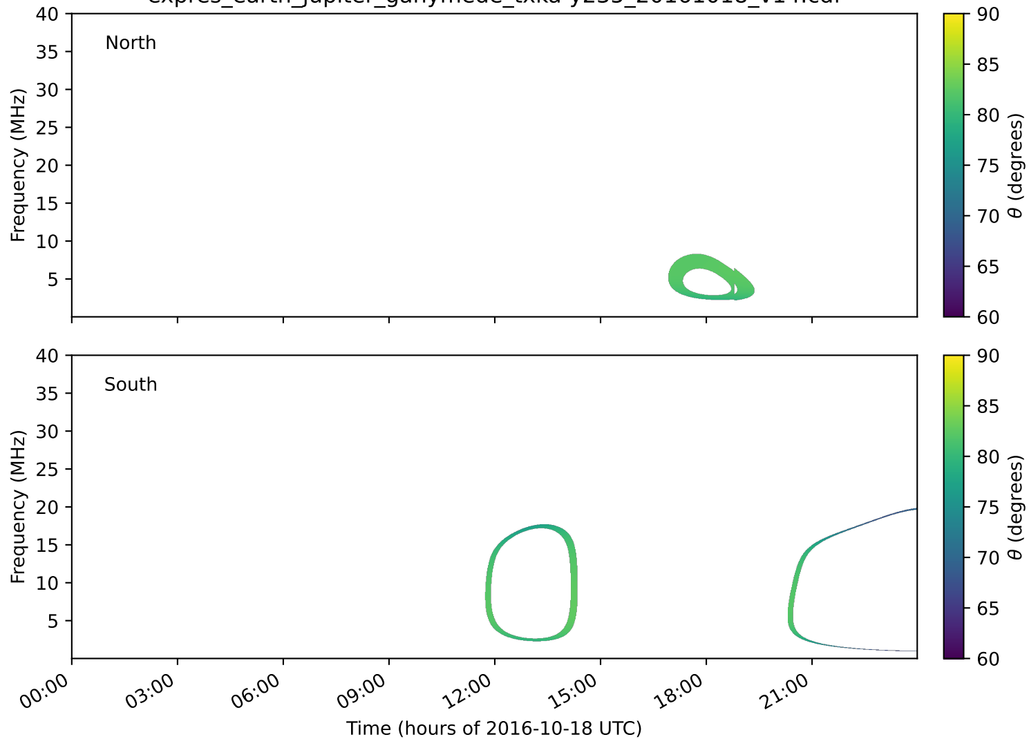
expres_earth_jupiter_ganymede_txka-y235_20161018_v14.cdf
