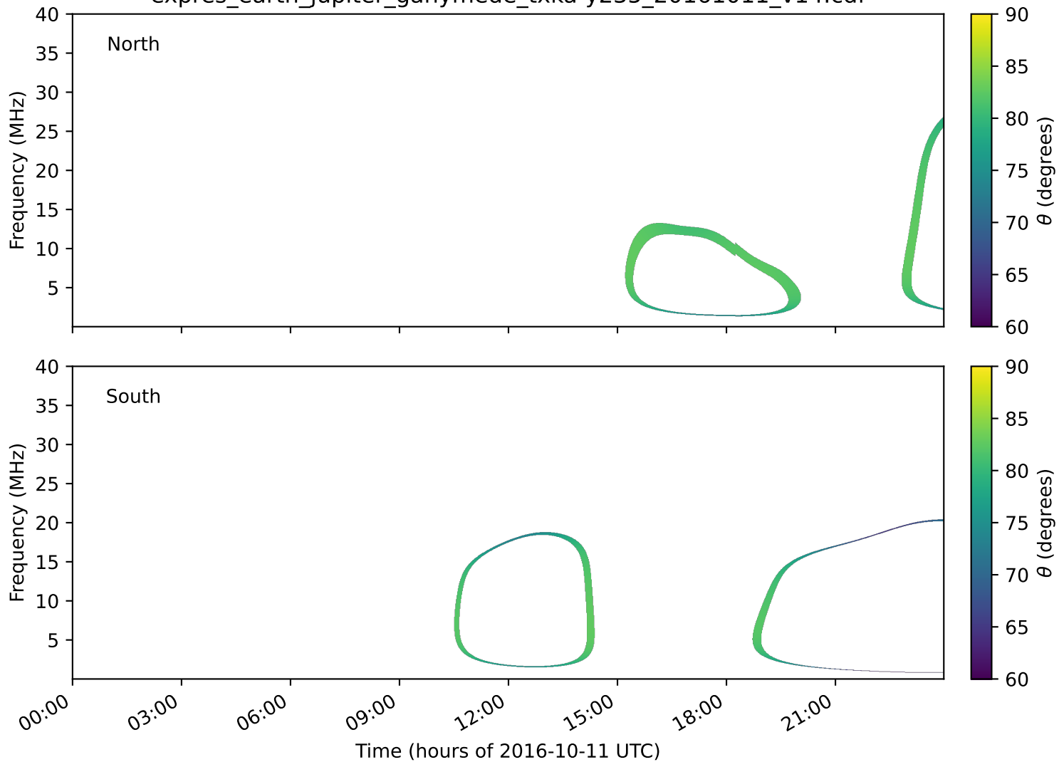
expres_earth_jupiter_ganymede_txka-y235_20161011_v14.cdf
