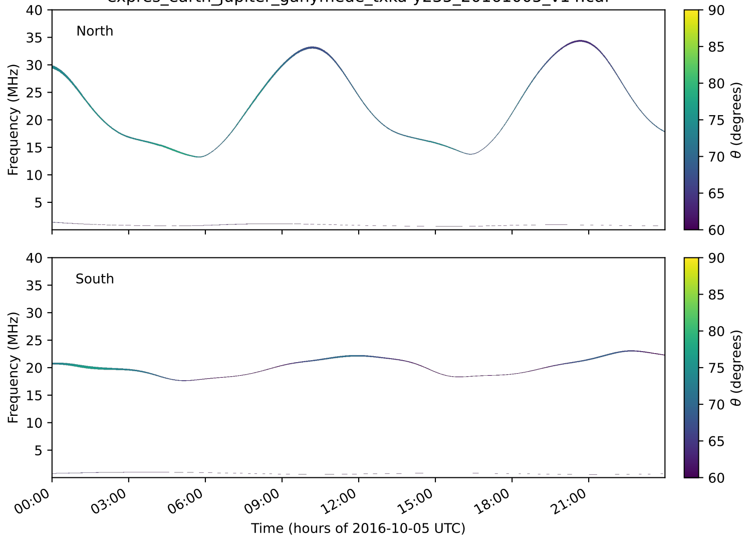
expres_earth_jupiter_ganymede_txka-y235_20161005_v14.cdf
