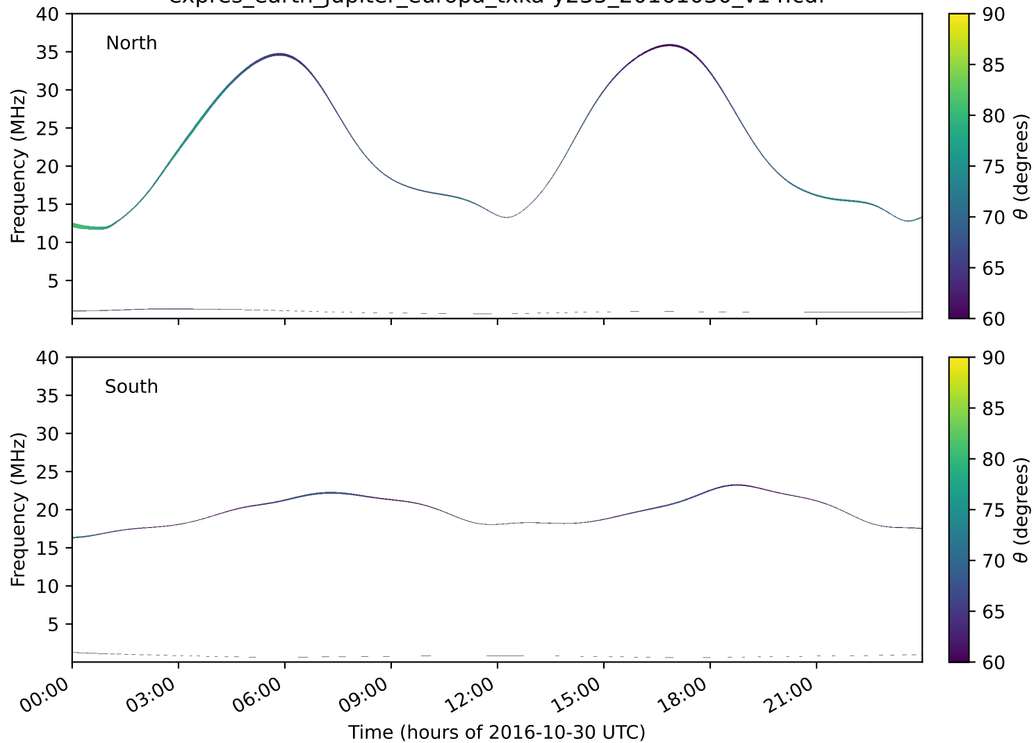
expres_earth_jupiter_europa_txka-y235_20161030_v14.cdf
