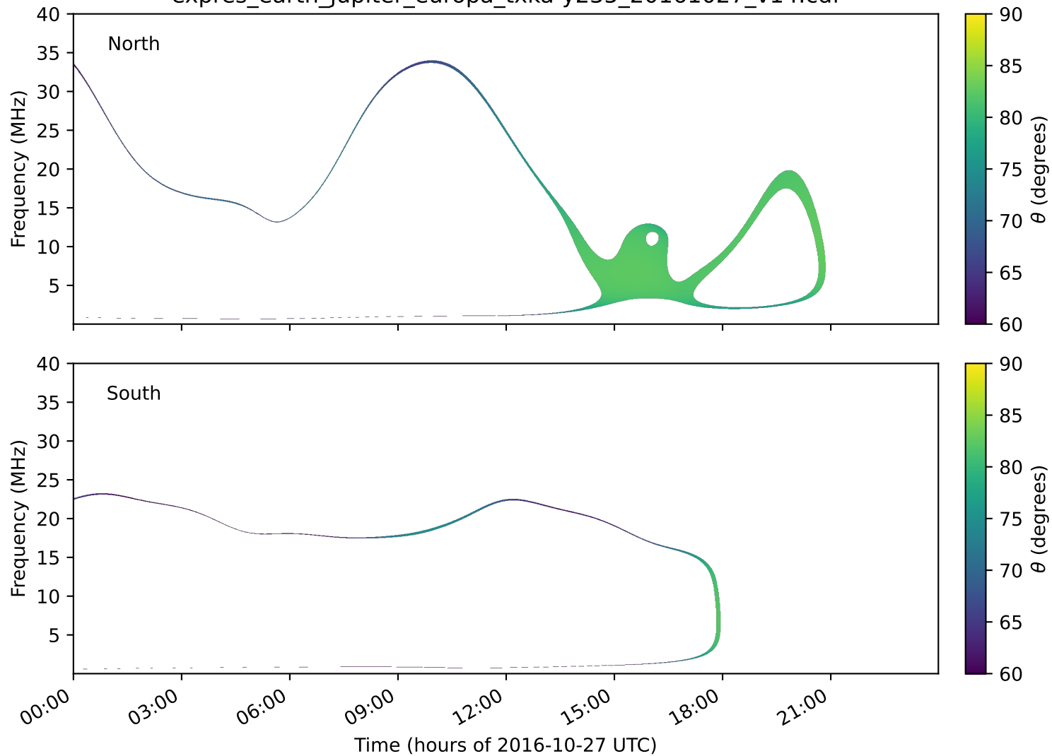
expres_earth_jupiter_europa_txka-y235_20161027_v14.cdf
