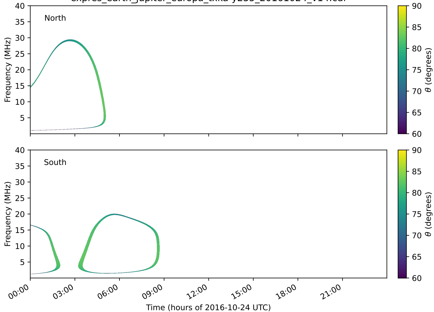
expres_earth_jupiter_europa_txka-y235_20161024_v14.cdf
