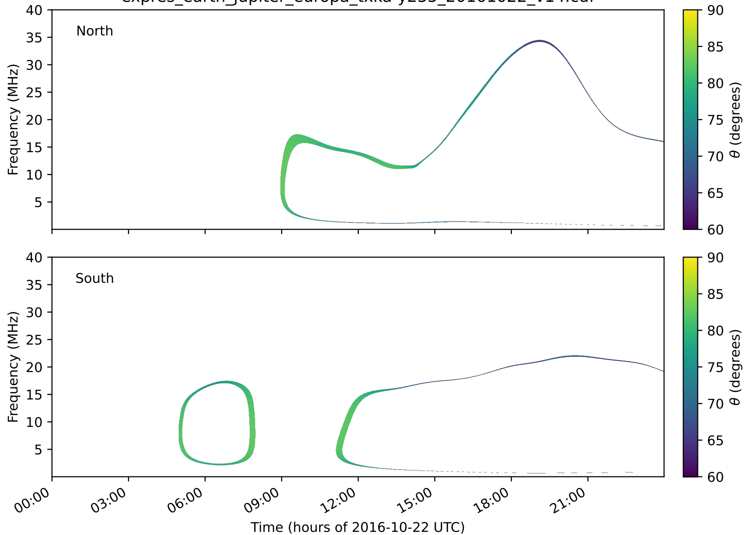
expres_earth_jupiter_europa_txka-y235_20161022_v14.cdf
