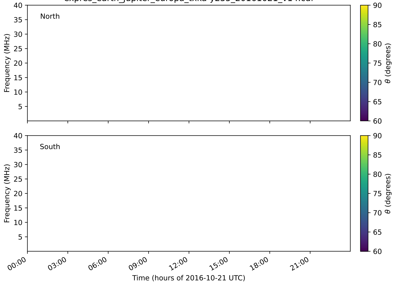
expres_earth_jupiter_europa_txka-y235_20161021_v14.cdf
