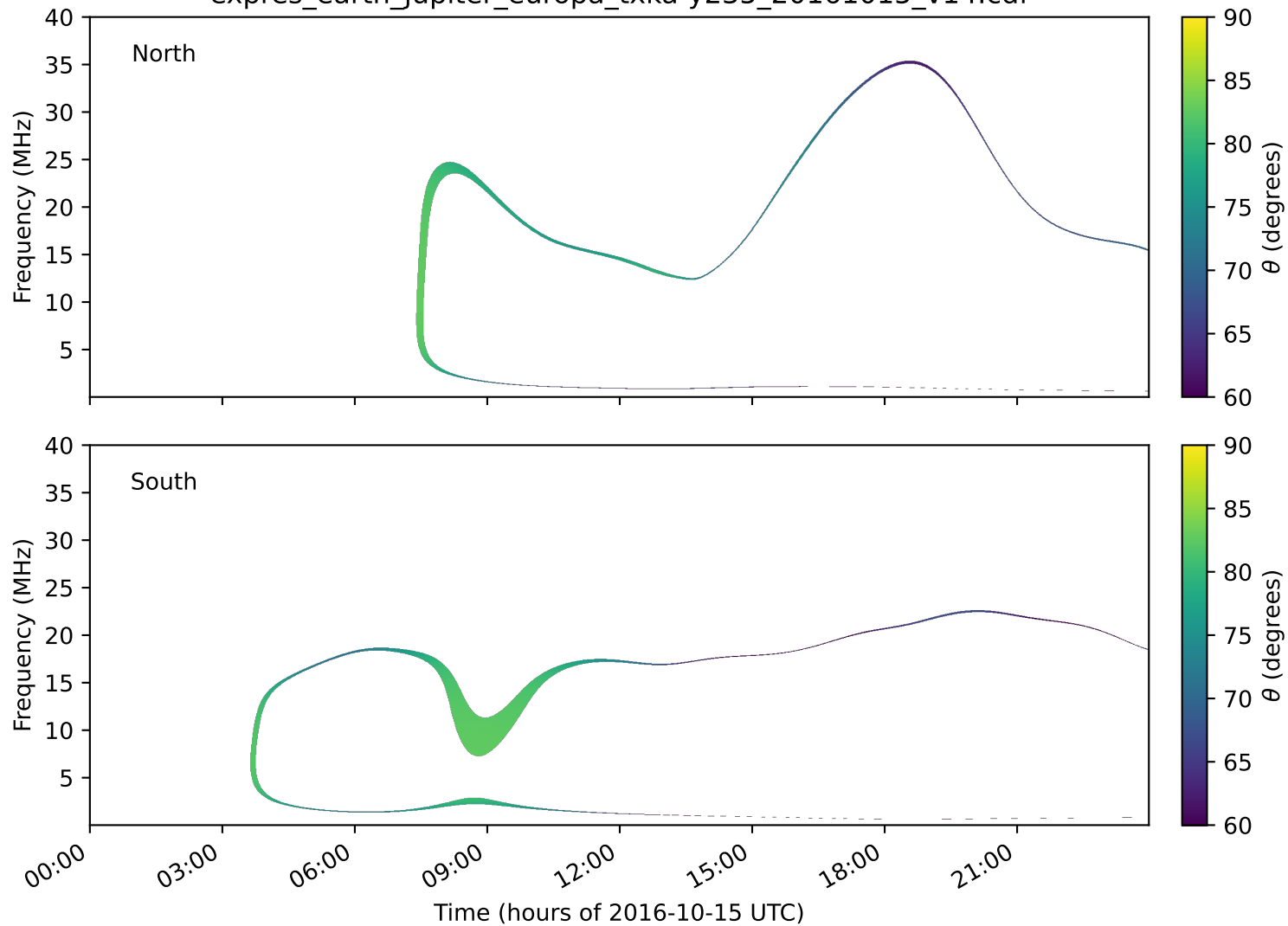
expres_earth_jupiter_europa_txka-y235_20161015_v14.cdf
