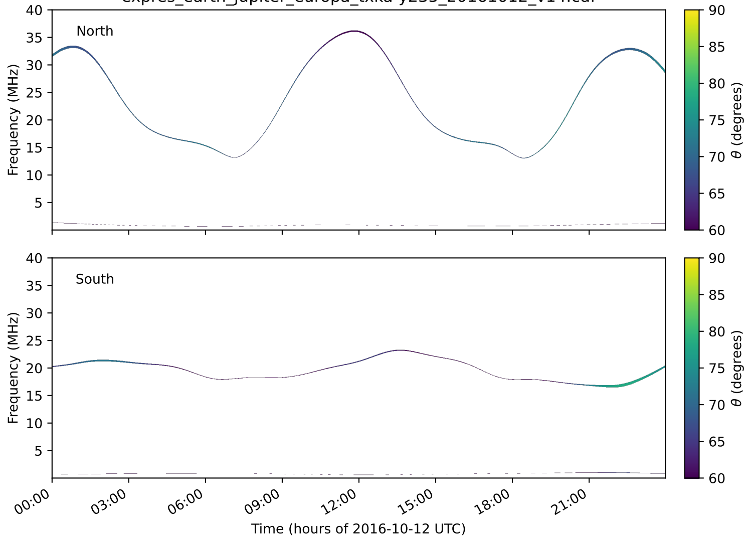
expres_earth_jupiter_europa_txka-y235_20161012_v14.cdf
