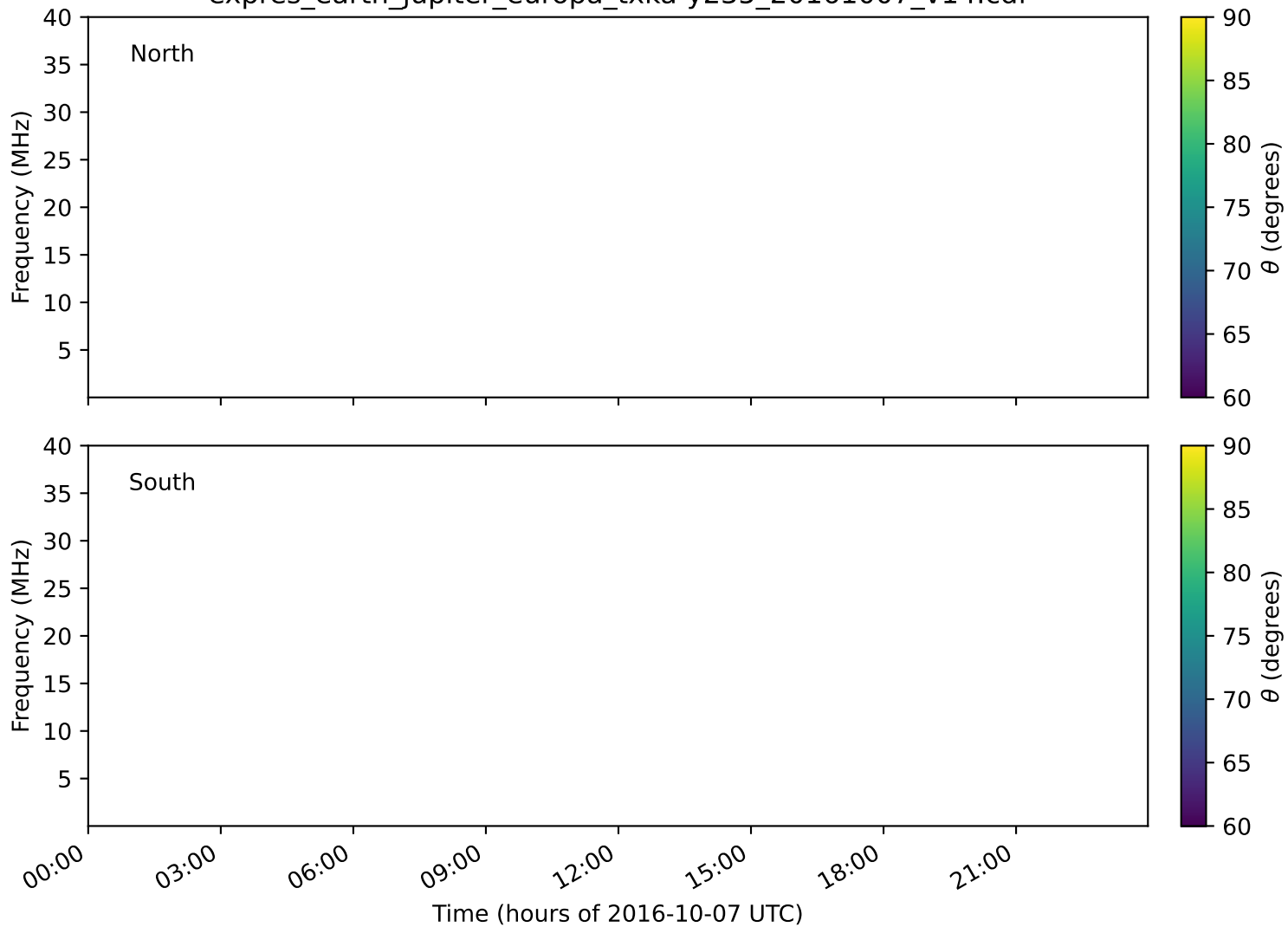
expres_earth_jupiter_europa_txka-y235_20161007_v14.cdf
