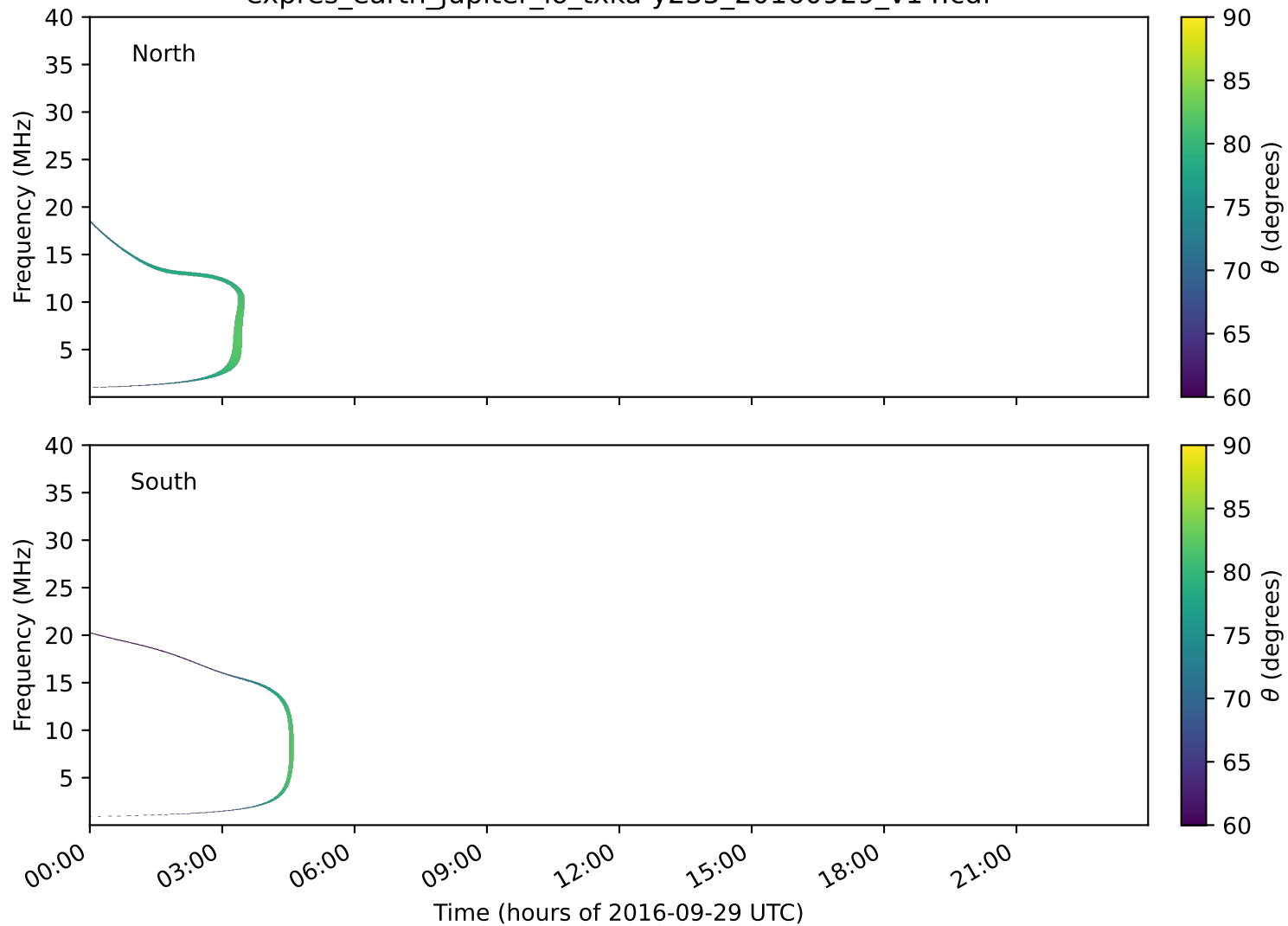
expres_earth_jupiter_io_txka-y235_20160929_v14.cdf
