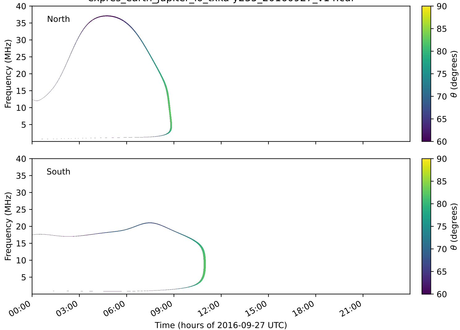
expres_earth_jupiter_io_txka-y235_20160927_v14.cdf
