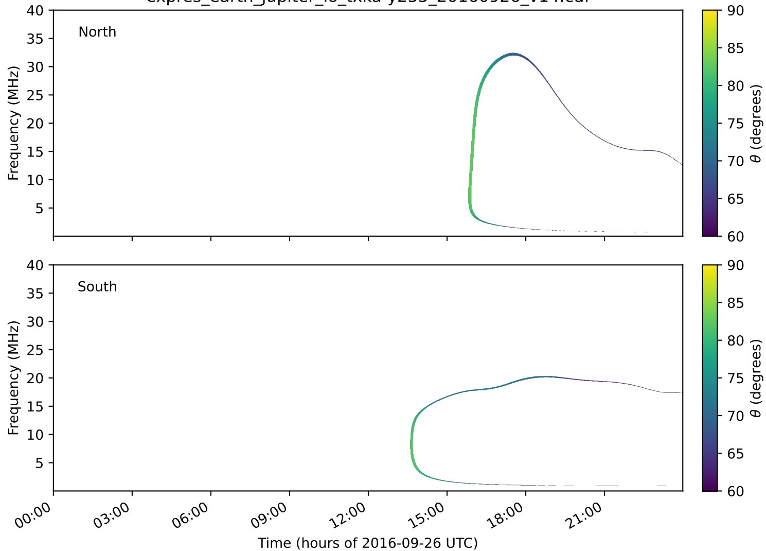
expres_earth_jupiter_io_txka-y235_20160926_v14.cdf
