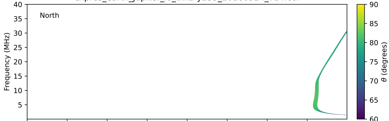
expres_earth_jupiter_io_txka-y235_20160924_v14.cdf
