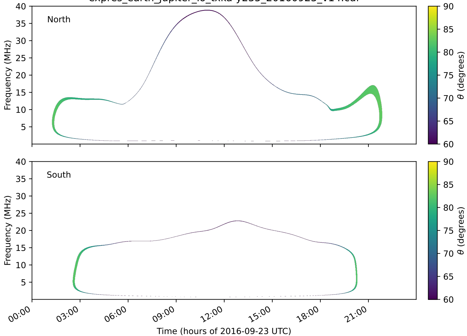
expres_earth_jupiter_io_txka-y235_20160923_v14.cdf
