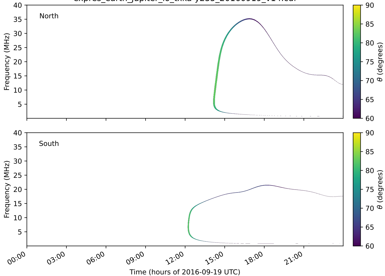
expres_earth_jupiter_io_txka-y235_20160919_v14.cdf
