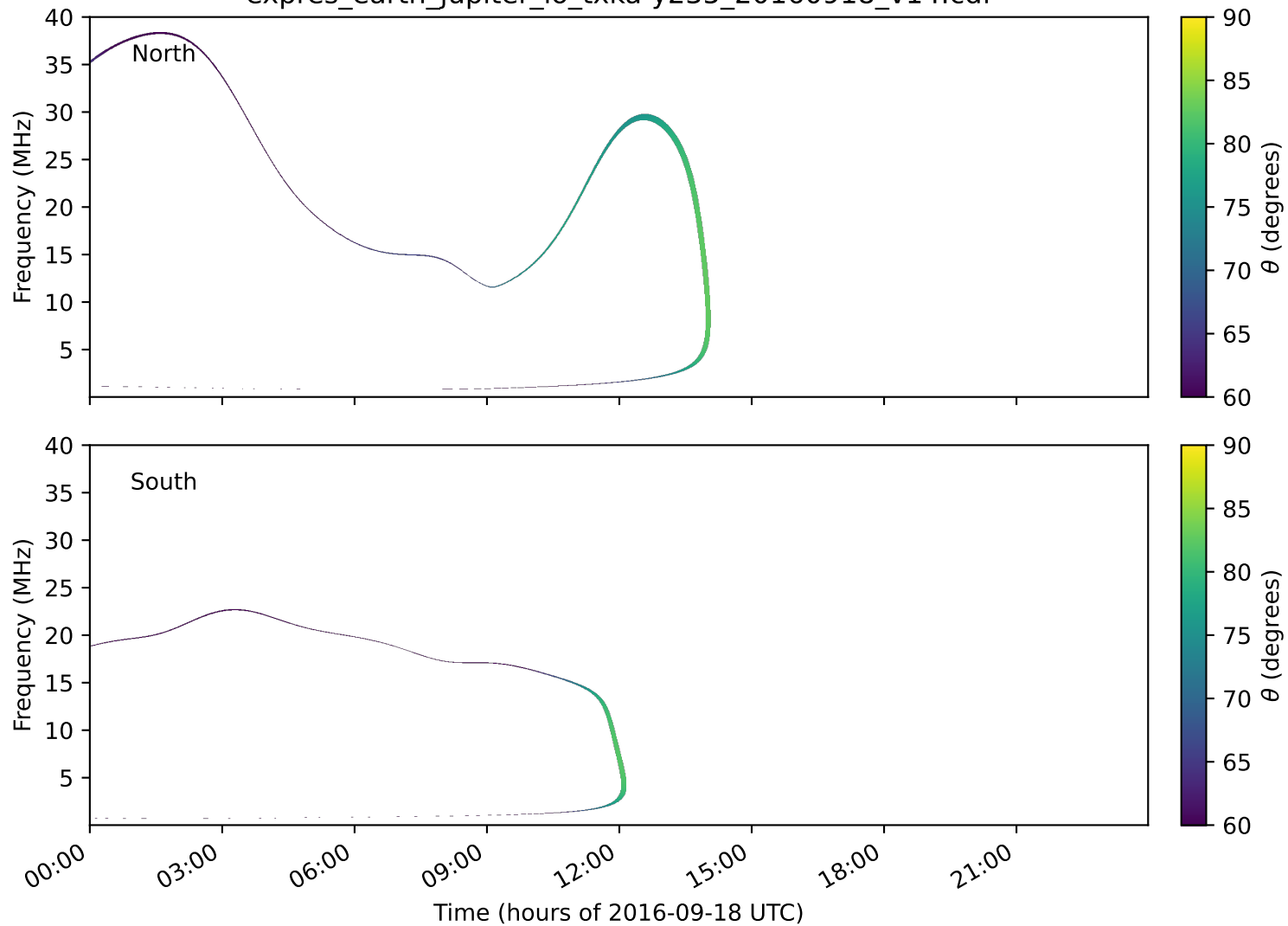
expres_earth_jupiter_io_txka-y235_20160918_v14.cdf
