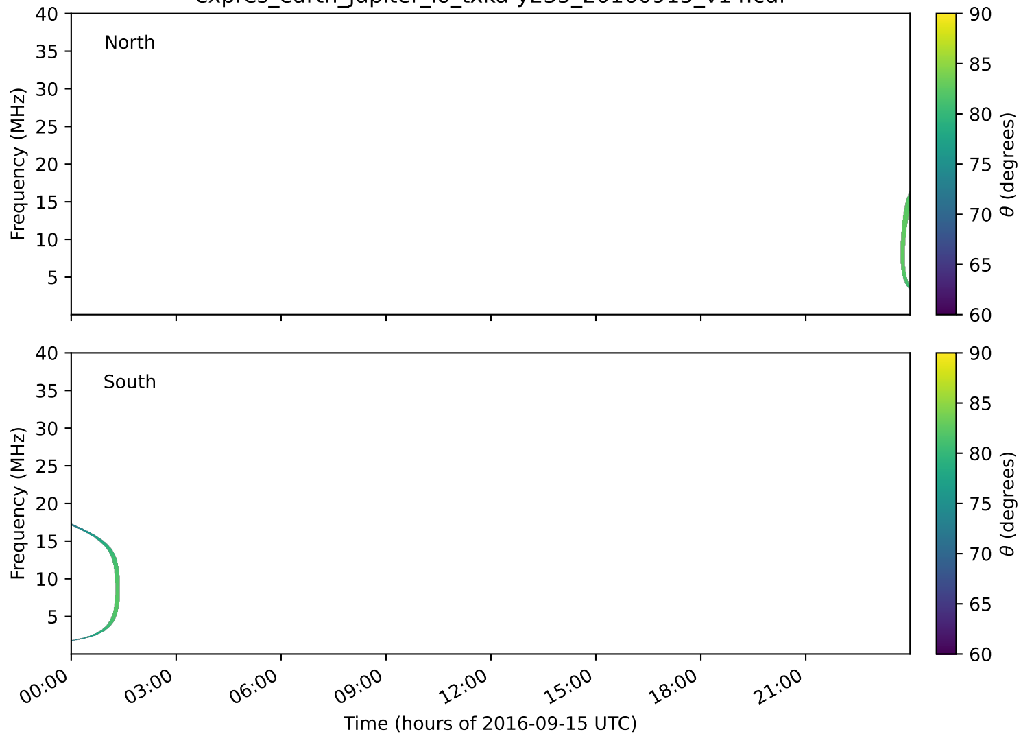
expres_earth_jupiter_io_txka-y235_20160915_v14.cdf
