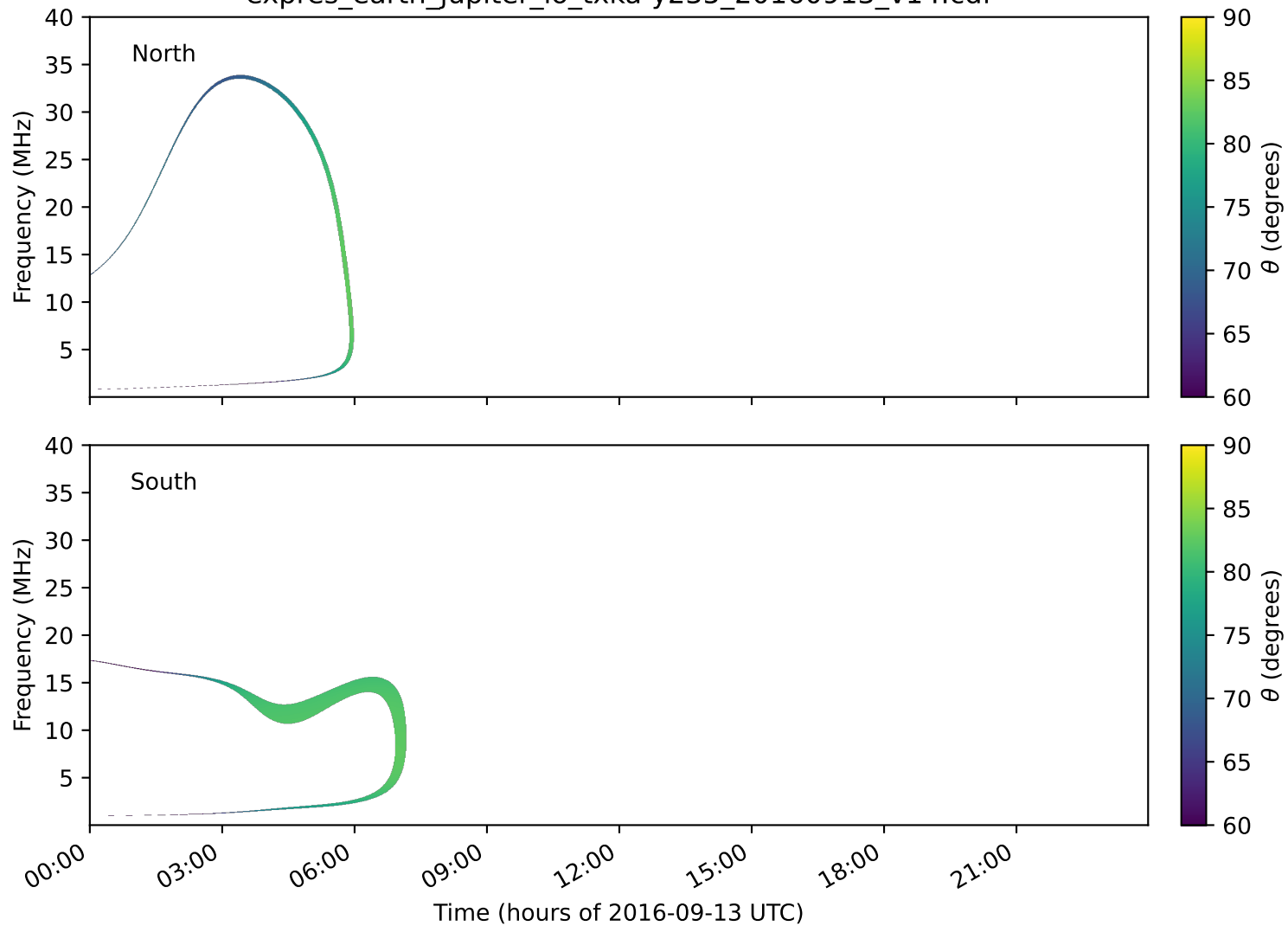
expres_earth_jupiter_io_txka-y235_20160913_v14.cdf
