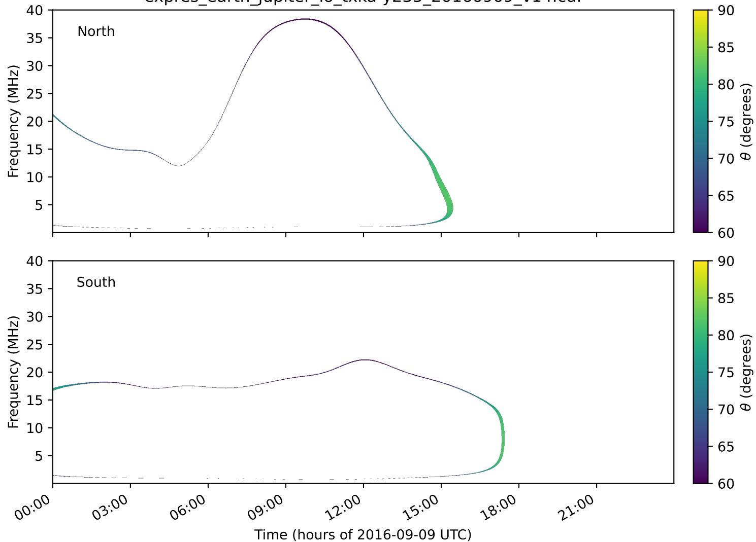
expres_earth_jupiter_io_txka-y235_20160909_v14.cdf
