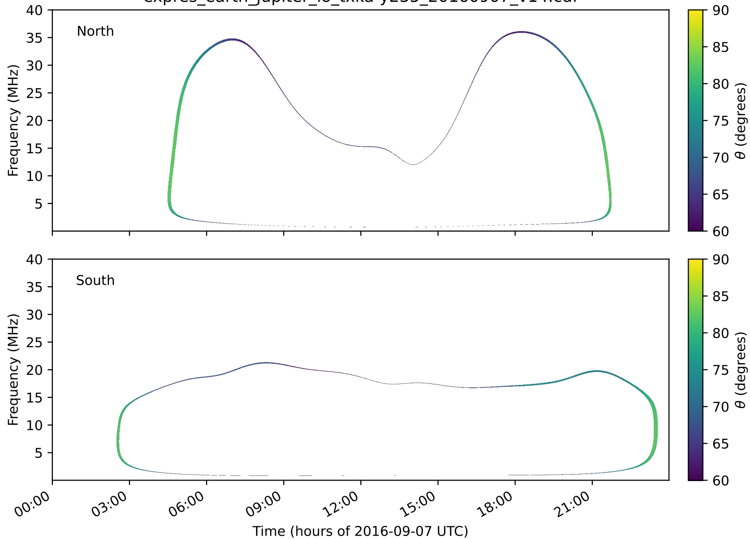
expres_earth_jupiter_io_txka-y235_20160907_v14.cdf
