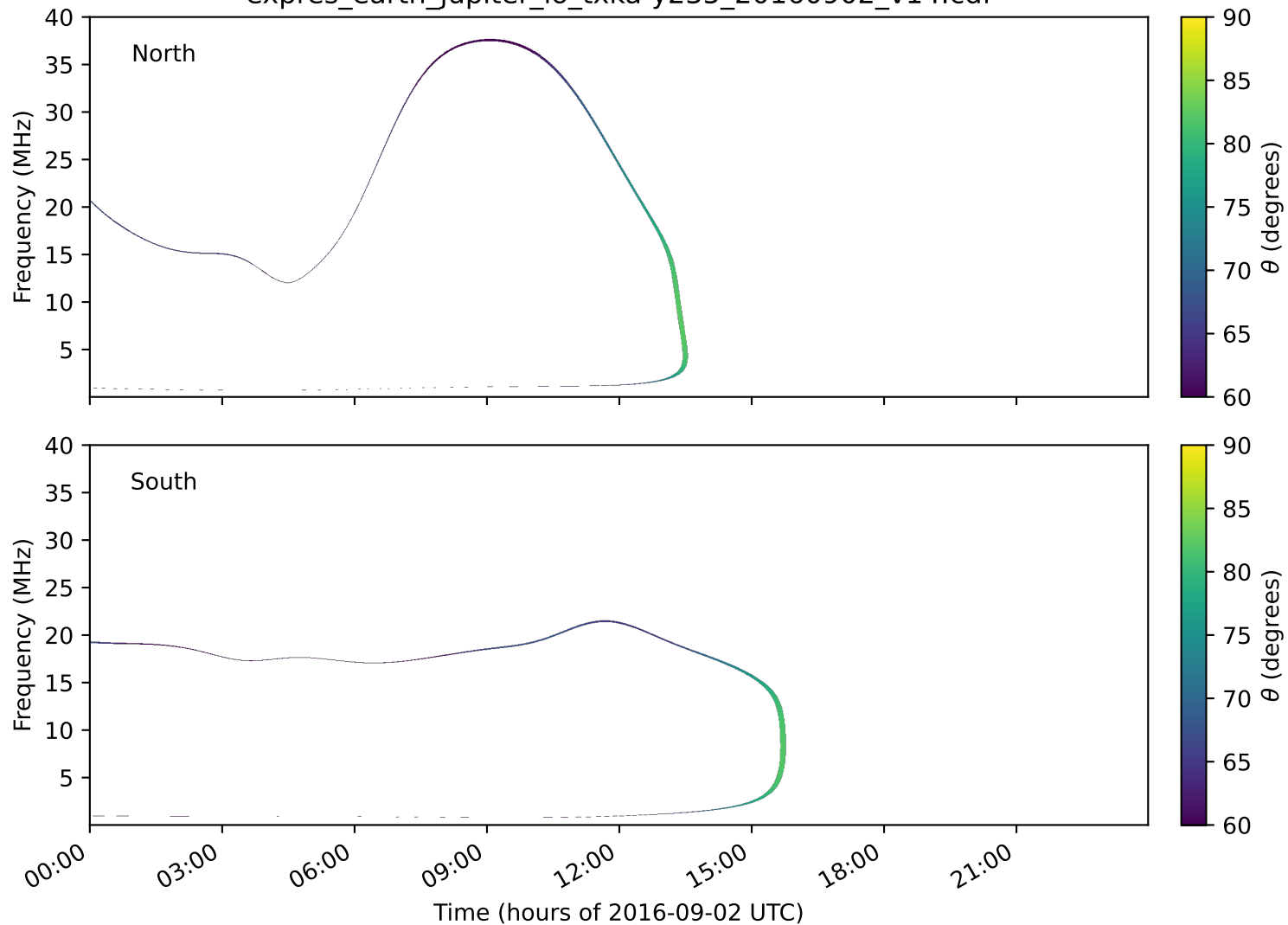
expres_earth_jupiter_io_txka-y235_20160902_v14.cdf
