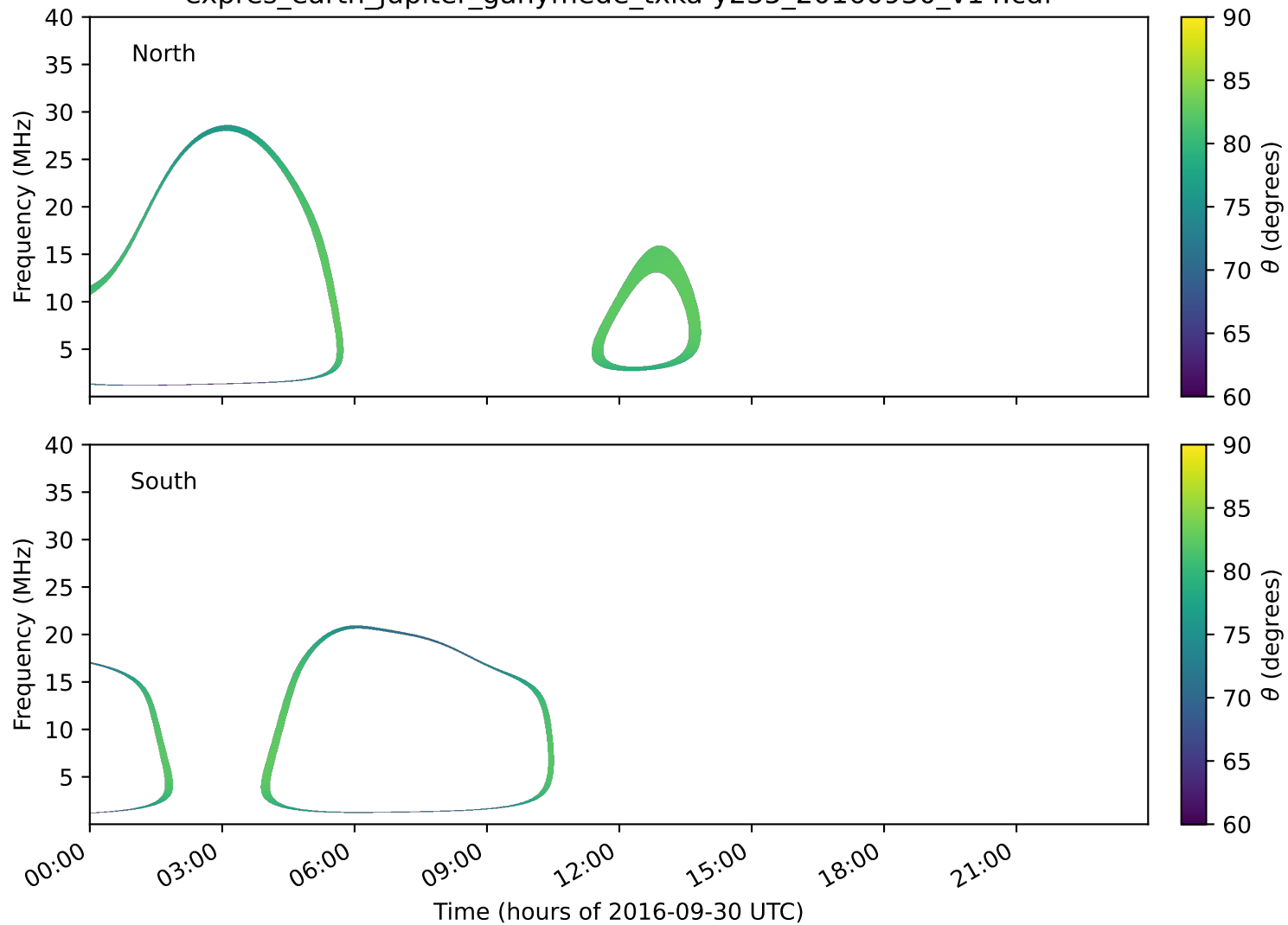
expres_earth_jupiter_ganymede_txka-y235_20160930_v14.cdf
