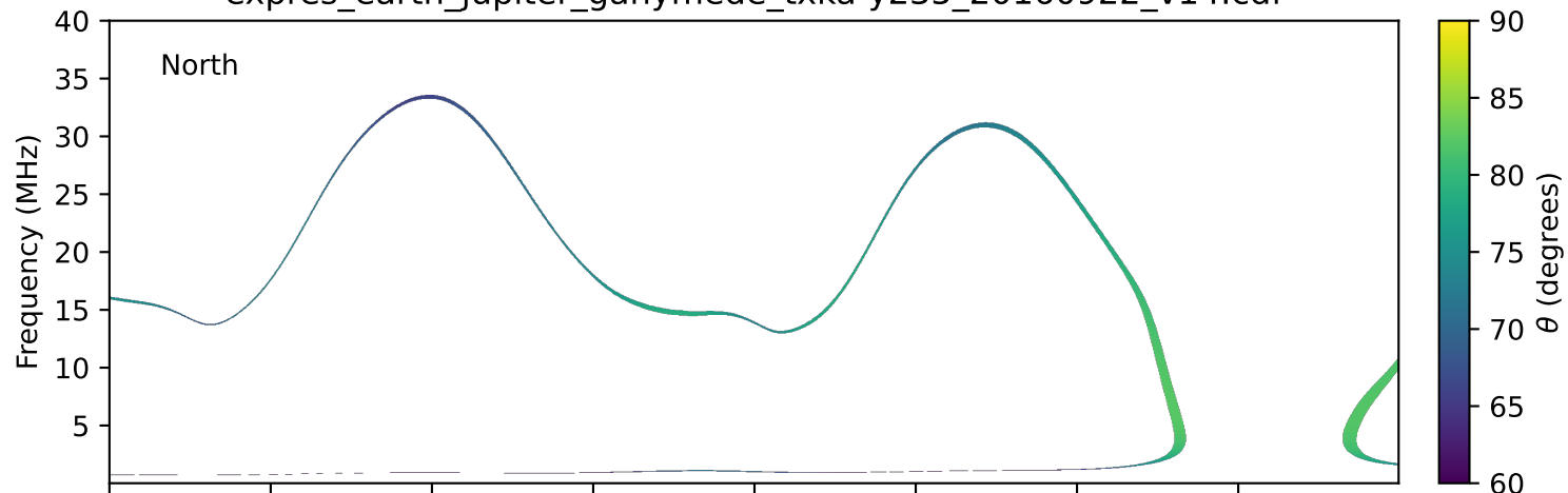
expres_earth_jupiter_ganymede_txka-y235_20160922_v14.cdf
