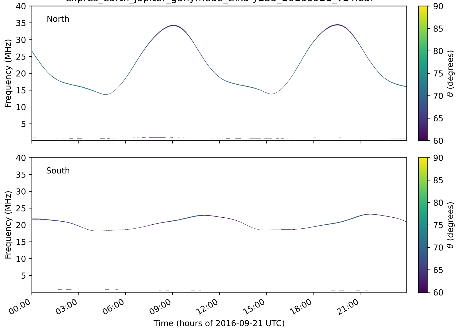
expres_earth_jupiter_ganymede_txka-y235_20160921_v14.cdf
