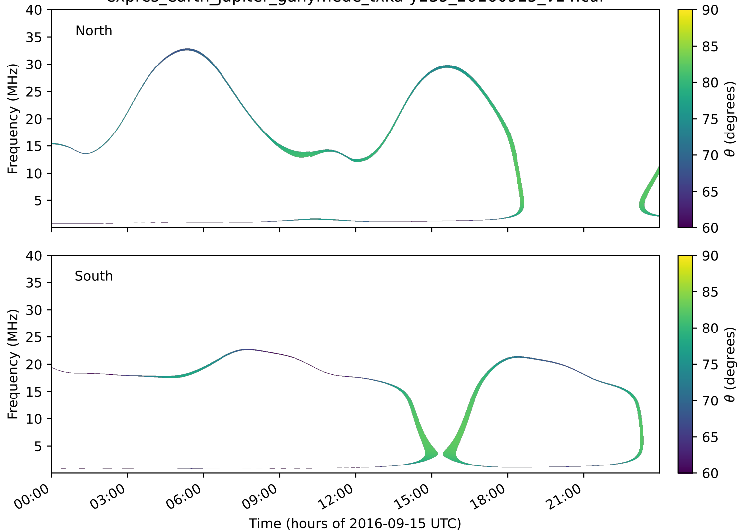
expres_earth_jupiter_ganymede_txka-y235_20160915_v14.cdf
