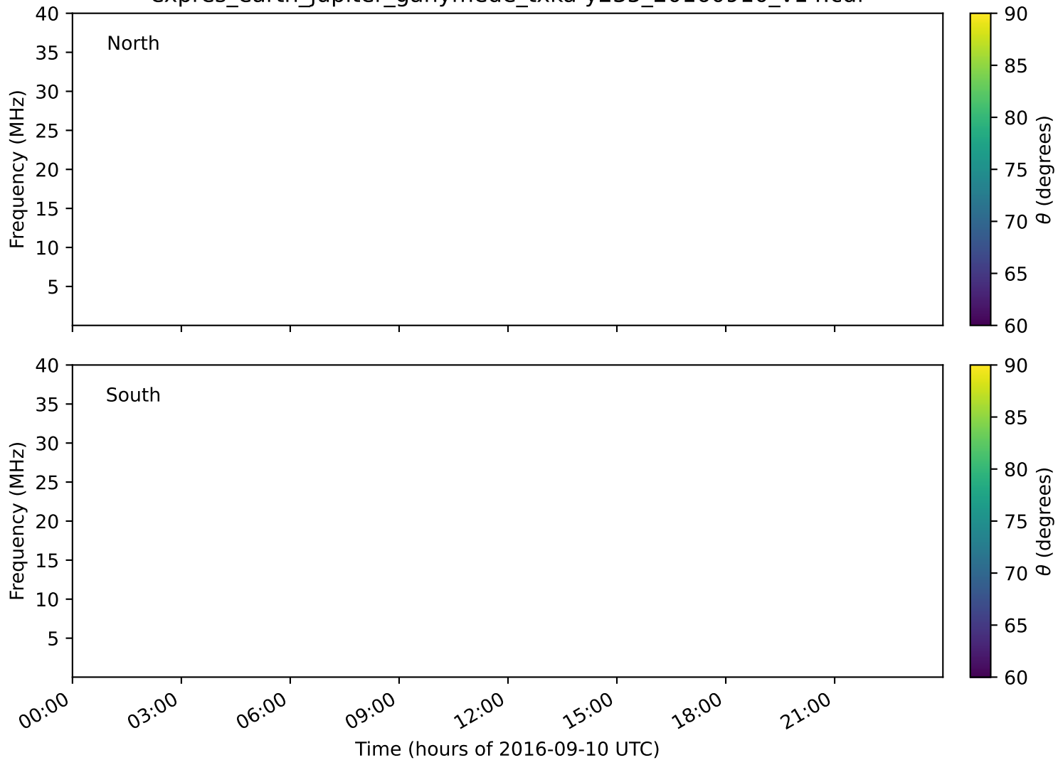
expres_earth_jupiter_ganymede_txka-y235_20160910_v14.cdf
