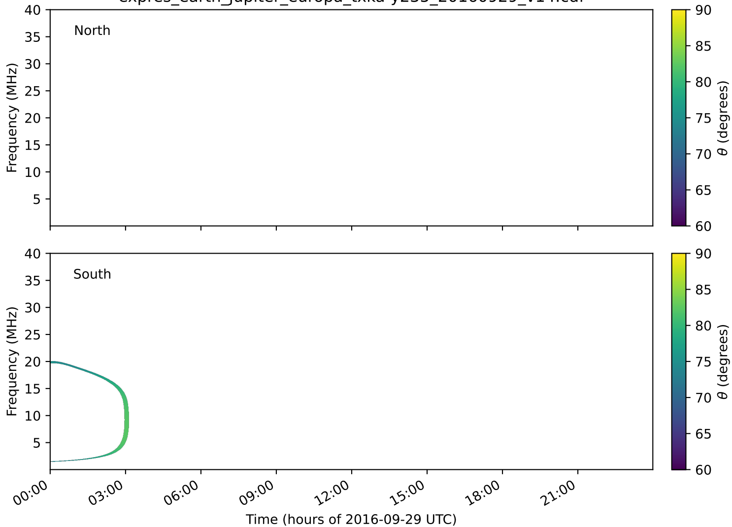
expres_earth_jupiter_europa_txka-y235_20160929_v14.cdf
