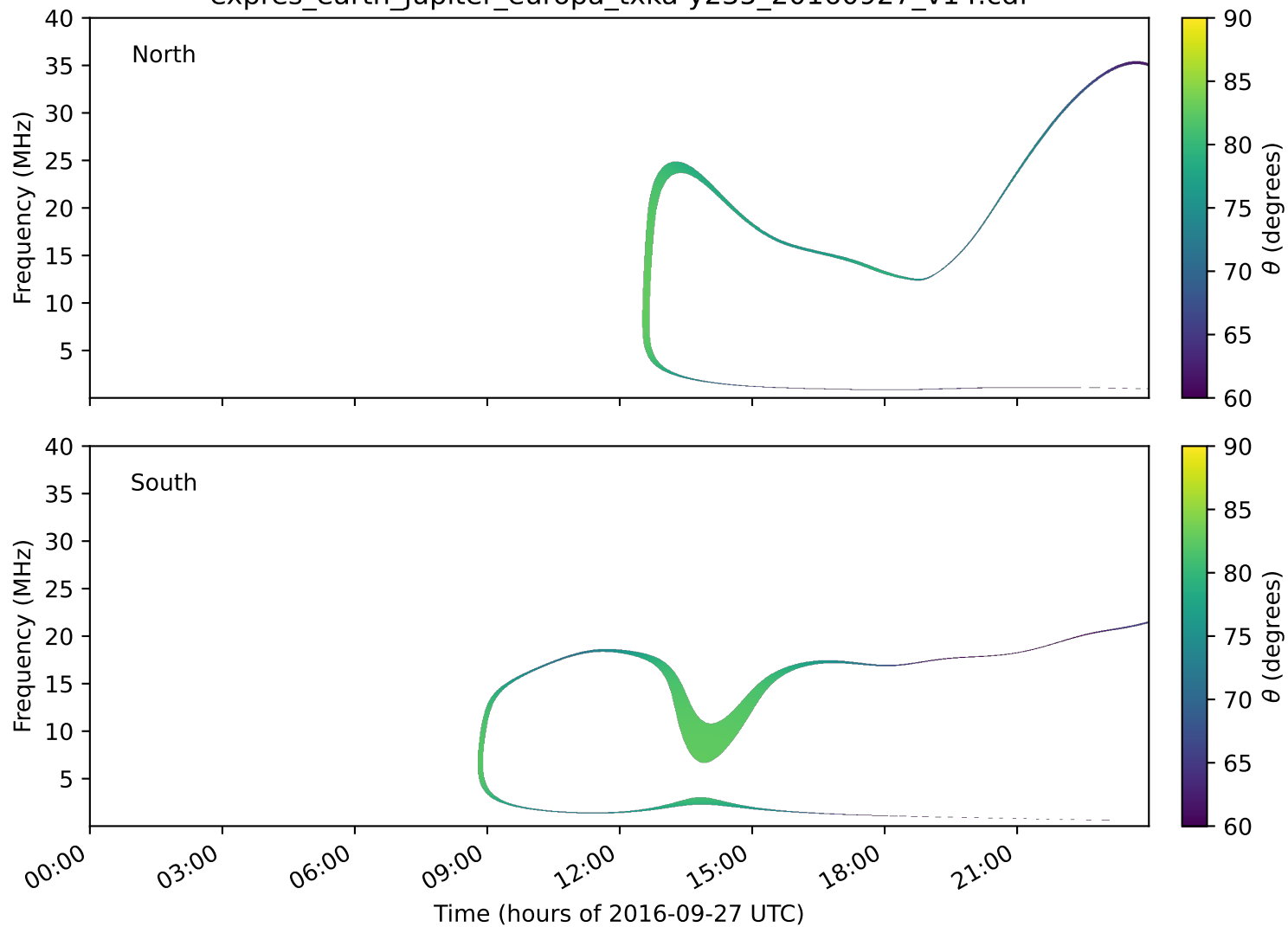
expres_earth_jupiter_europa_txka-y235_20160927_v14.cdf
