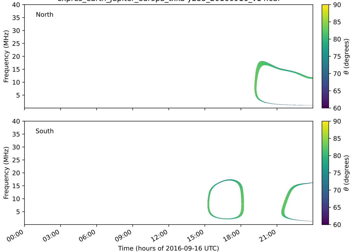
expres_earth_jupiter_europa_txka-y235_20160916_v14.cdf
