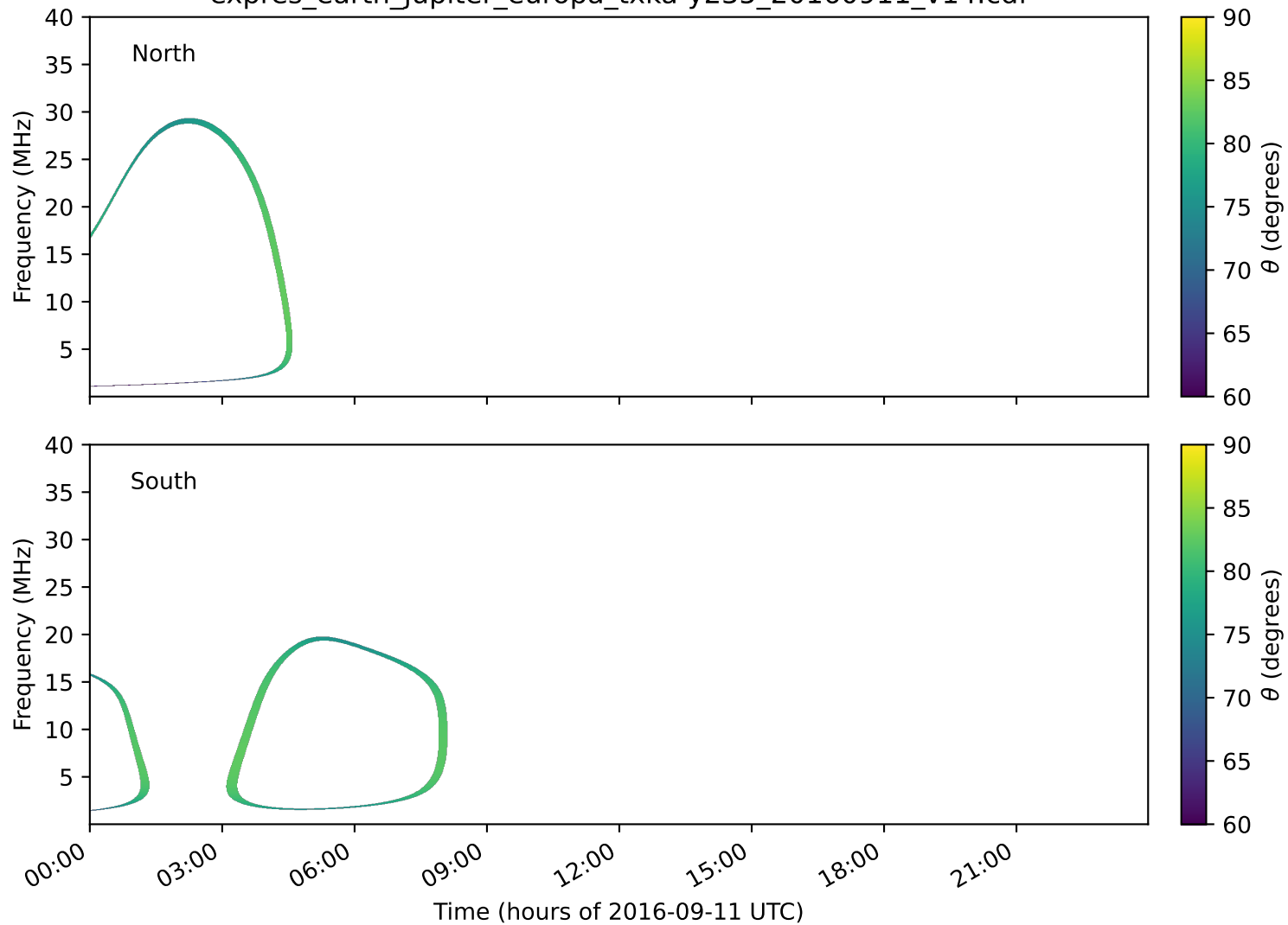
expres_earth_jupiter_europa_txka-y235_20160911_v14.cdf
