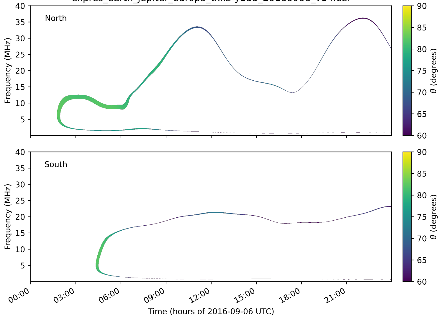
expres_earth_jupiter_europa_txka-y235_20160906_v14.cdf
