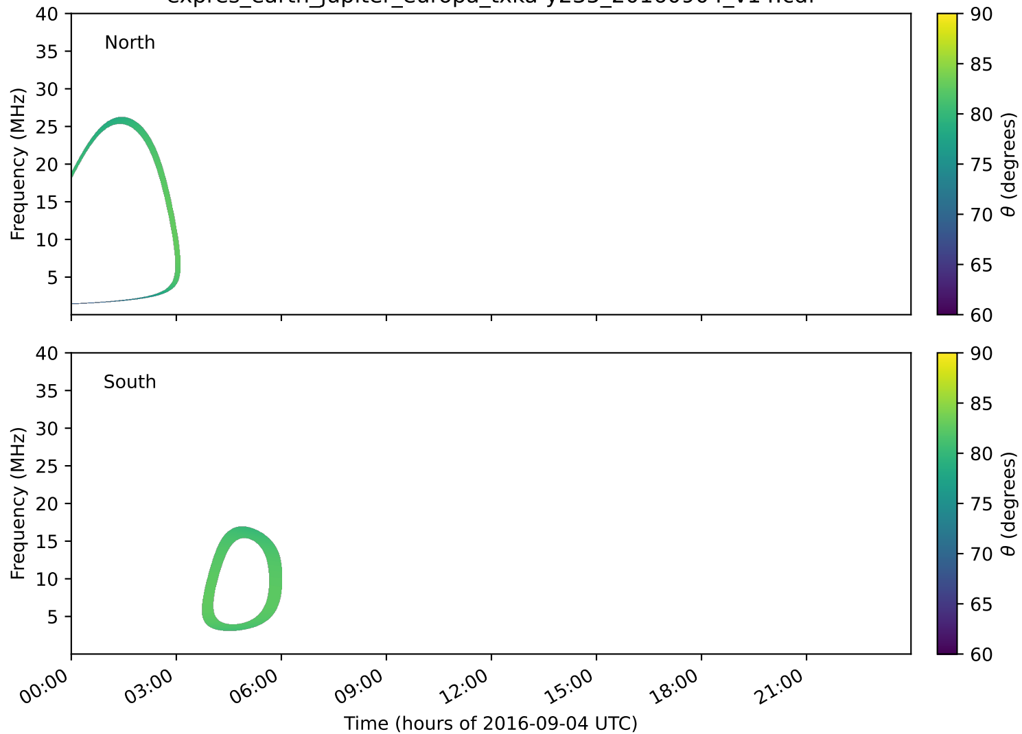
expres_earth_jupiter_europa_txka-y235_20160904_v14.cdf
