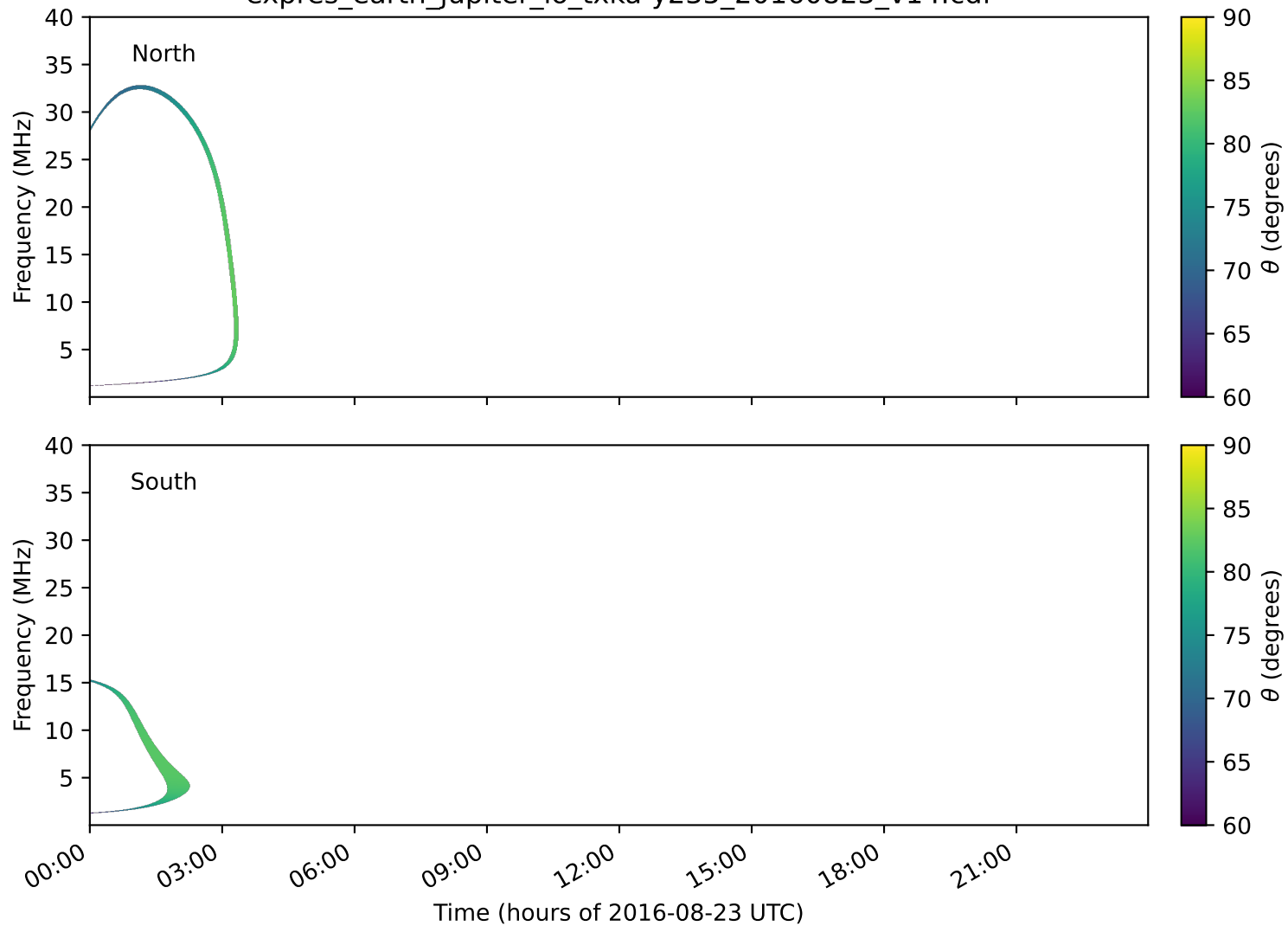
expres_earth_jupiter_io_txka-y235_20160823_v14.cdf
