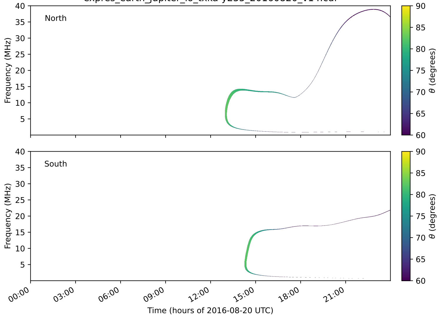
expres_earth_jupiter_io_txka-y235_20160820_v14.cdf
