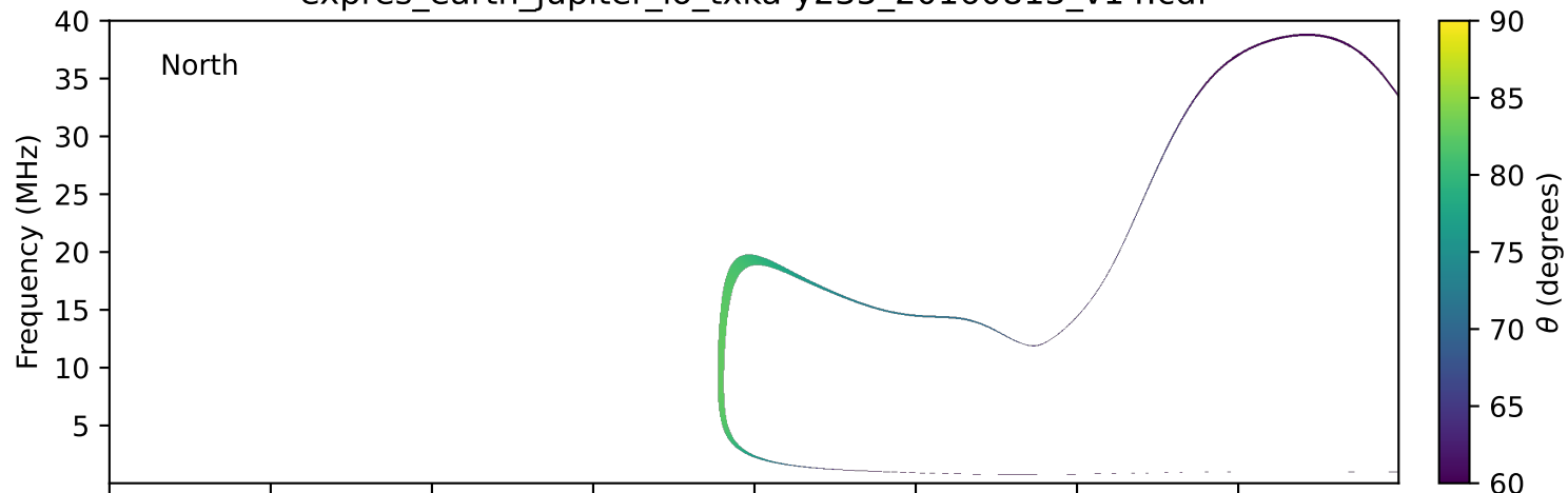
expres_earth_jupiter_io_txka-y235_20160813_v14.cdf
