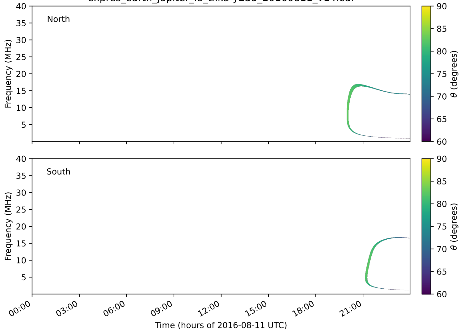
expres_earth_jupiter_io_txka-y235_20160811_v14.cdf
