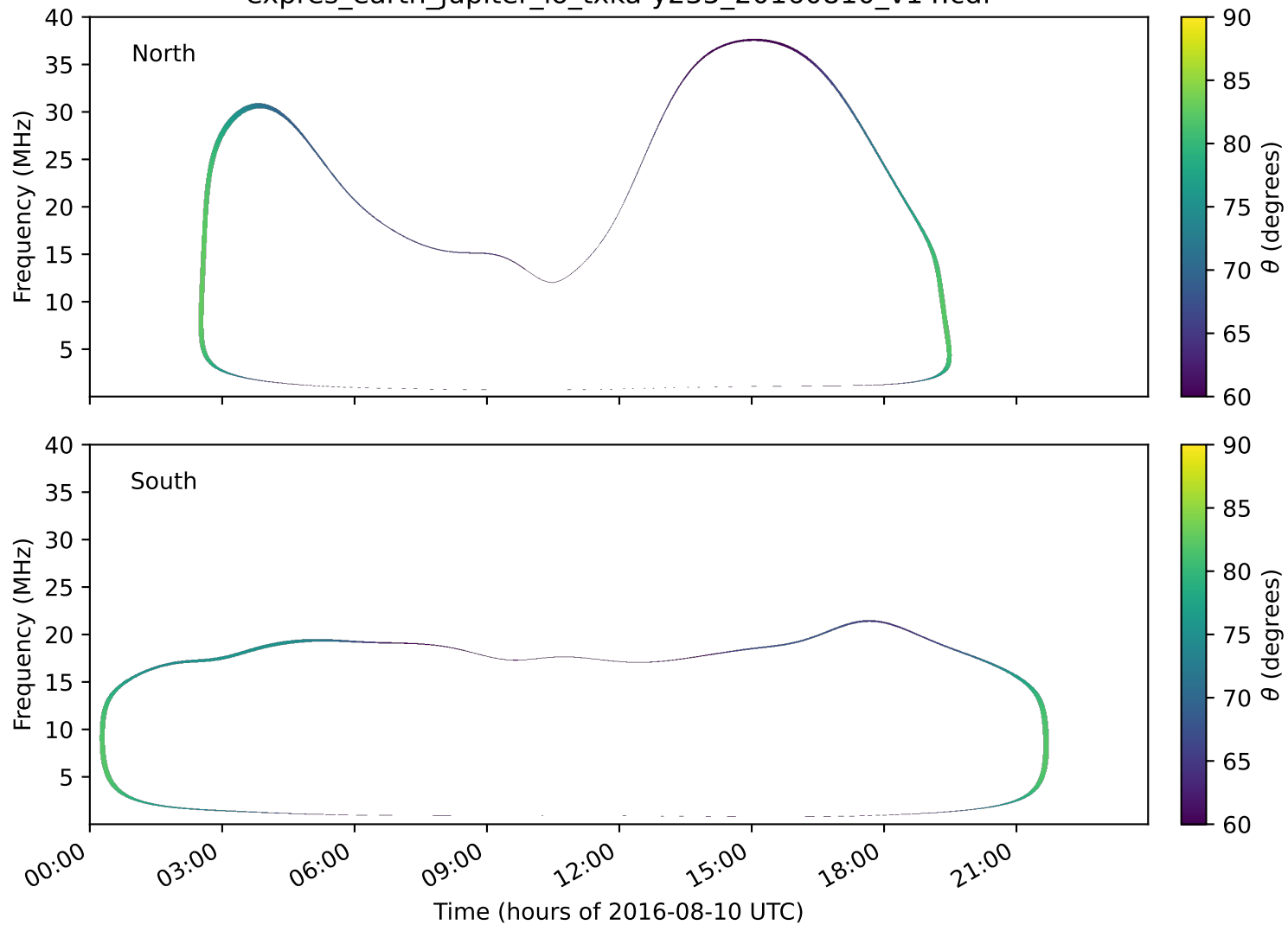
expres_earth_jupiter_io_txka-y235_20160810_v14.cdf
