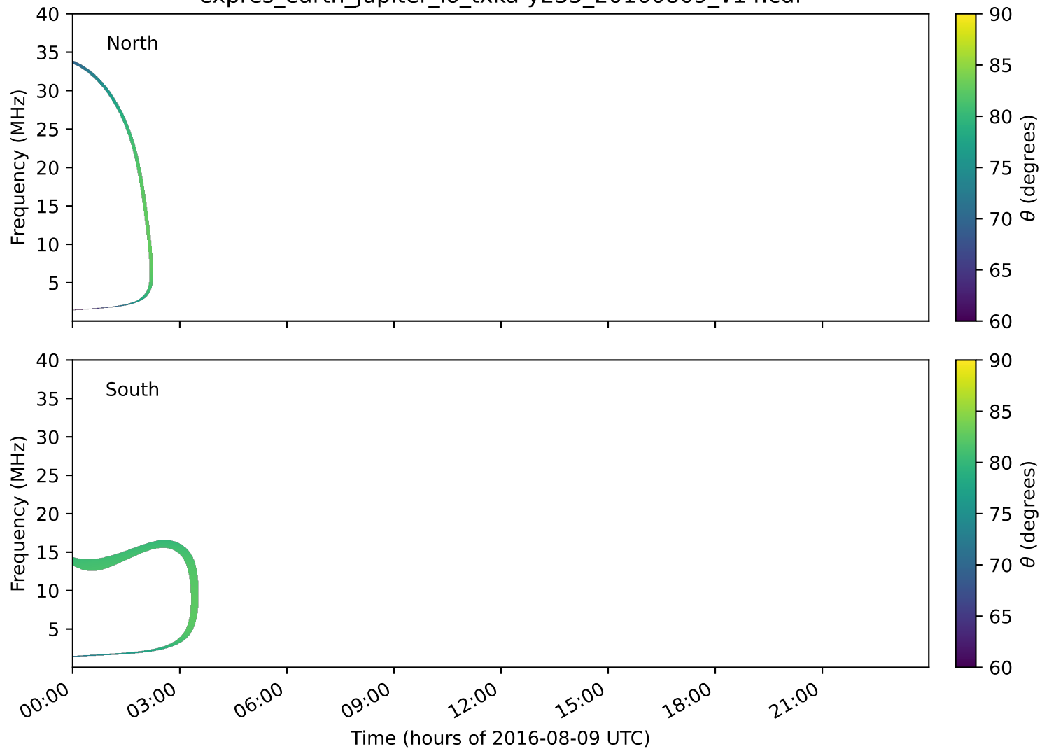
expres_earth_jupiter_io_txka-y235_20160809_v14.cdf
