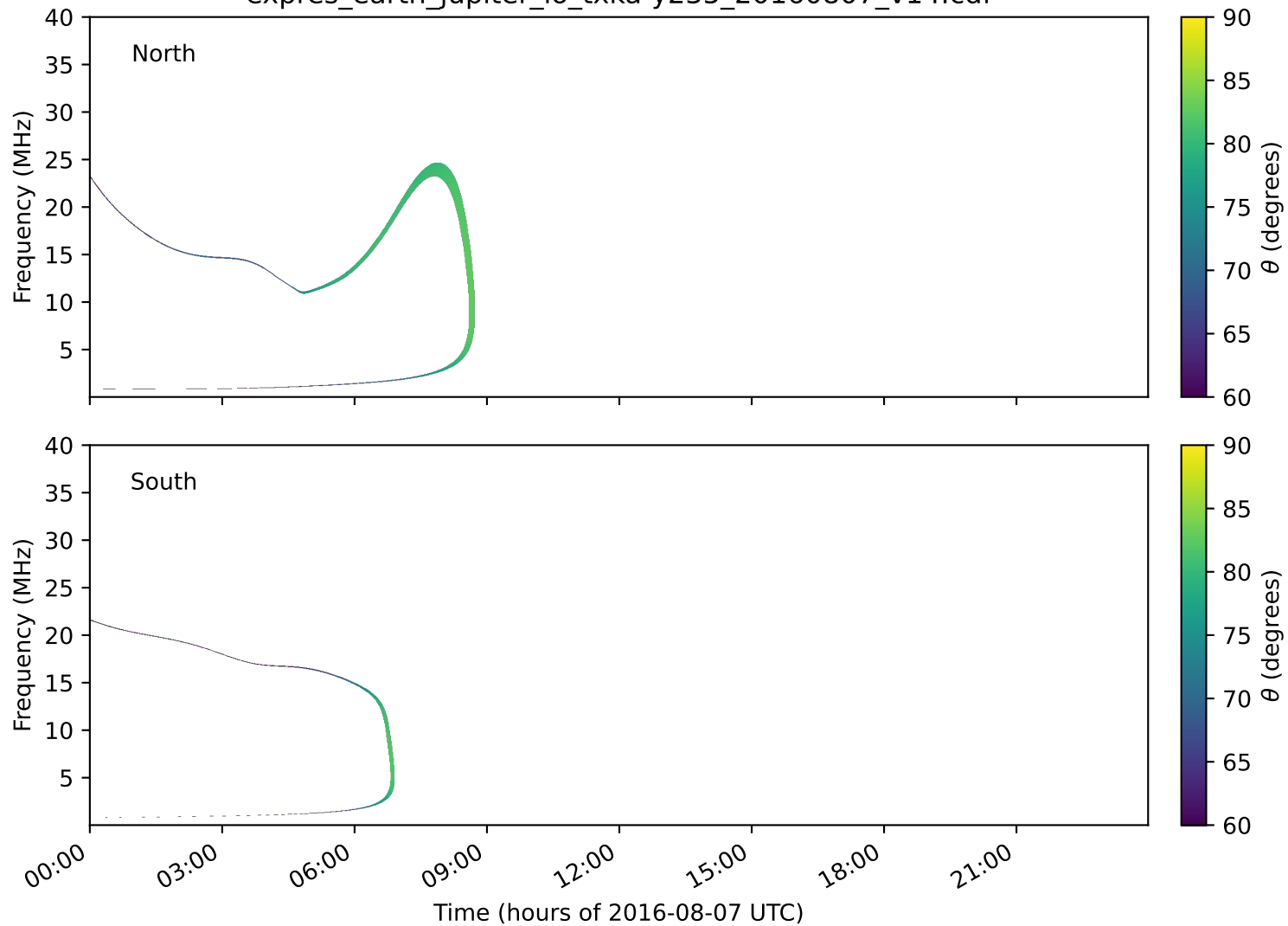
expres_earth_jupiter_io_txka-y235_20160807_v14.cdf
