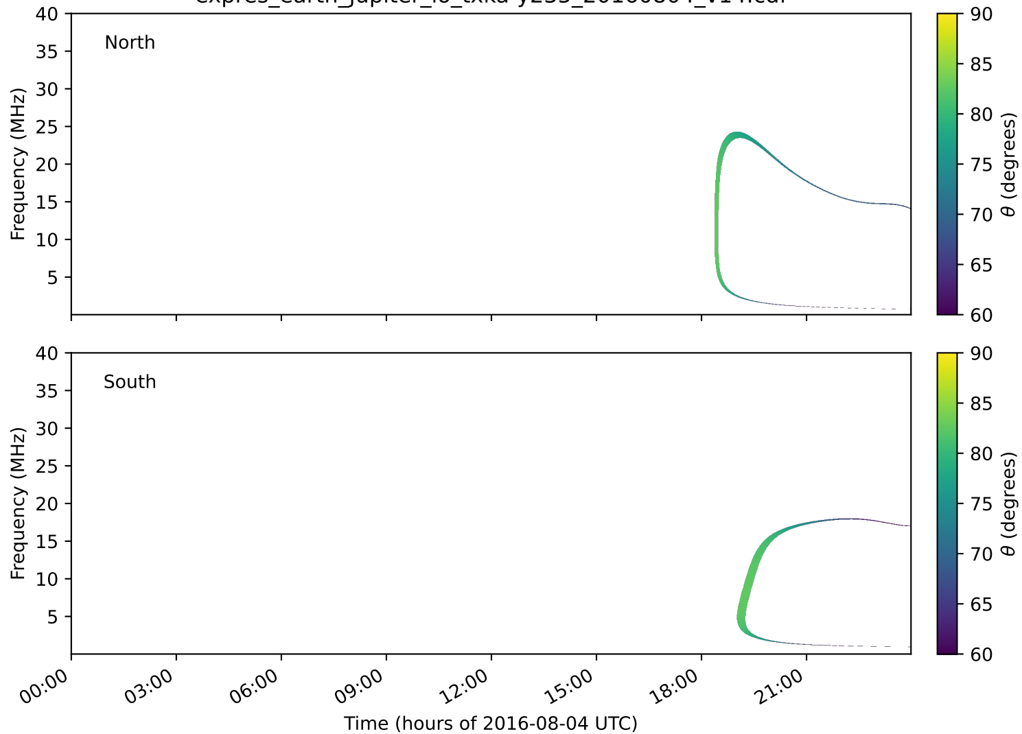
expres_earth_jupiter_io_txka-y235_20160804_v14.cdf
