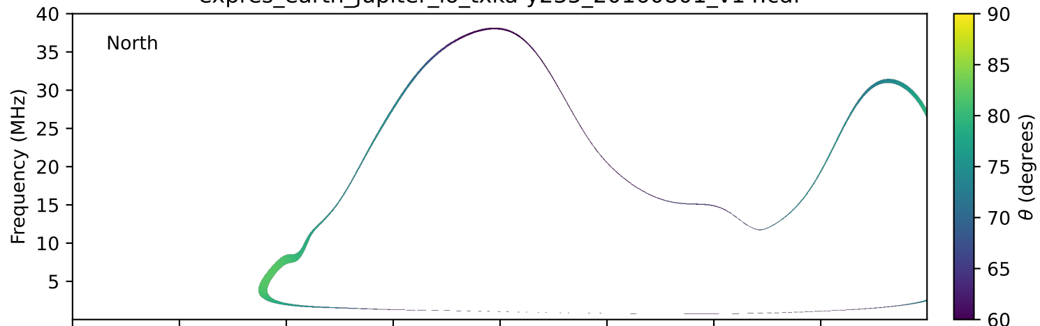
expres_earth_jupiter_io_txka-y235_20160801_v14.cdf
