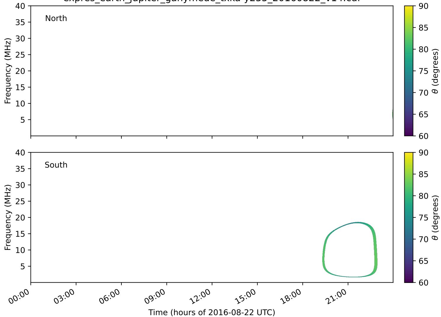
expres_earth_jupiter_ganymede_txka-y235_20160822_v14.cdf
