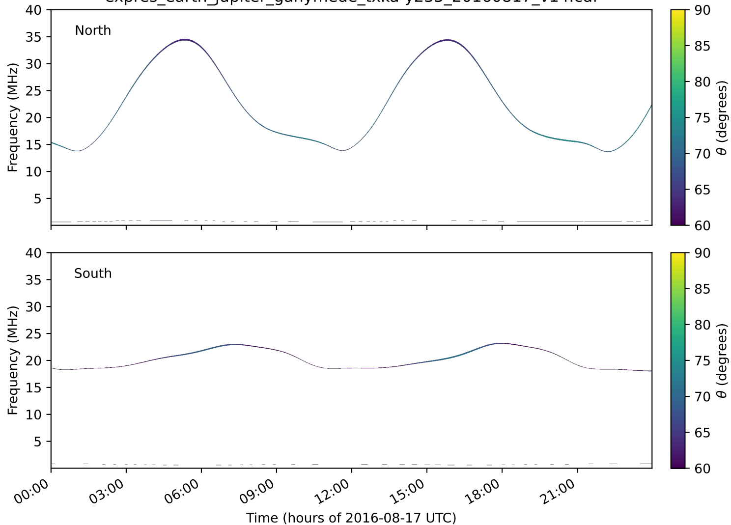
expres_earth_jupiter_ganymede_txka-y235_20160817_v14.cdf
